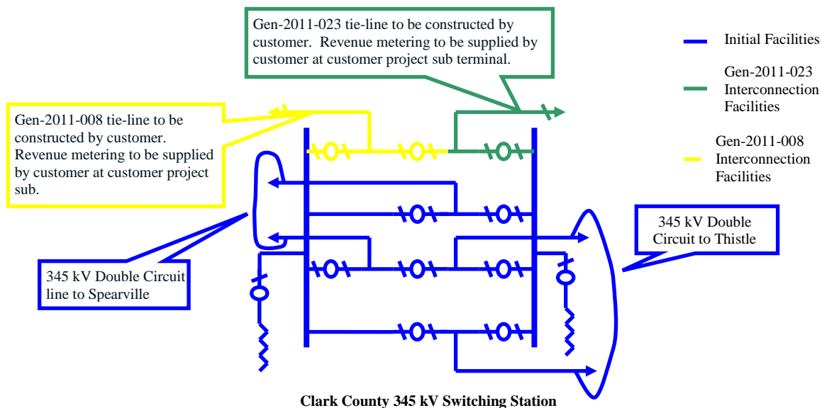
Figure 1 – Clark County Switching Station with Gen-2011-008 Interconnection
